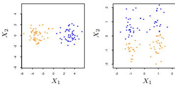
Figure 14.5: Simulated data: on the left, K-means clustering (with K=2 ) has been applied to the raw data. The two colors indicate the cluster memberships. On the right, the features were first standardized before clustering. This is equivalent to using feature weights 1/[2 \cdot \text{var}(X_j)] . The standardization has obscured the two well-separated groups. Note that each plot uses the same units in the horizontal and vertical axes.
