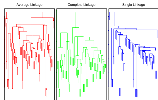
Figure 14.13: Dendrograms from agglomerative hier-
