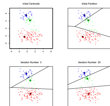
Figure 14.6: Successive iterations of the K-means clustering algorithm for the simulated data of Fig.
