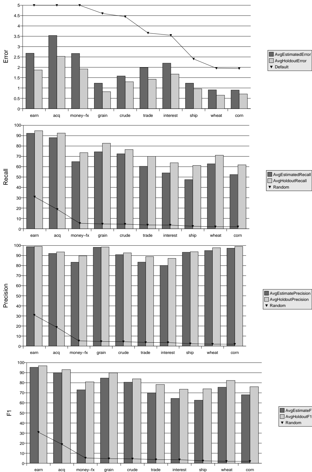
Figure 3: Diagrams comparing average \xi_\alpha -estimate ( \rho = 1 ) of the error, the recall, the precision, and the F1 -measure with the average true error, true recall, true precision, and true F1 measured on a holdout set for the ten most frequent Reuters categories.
