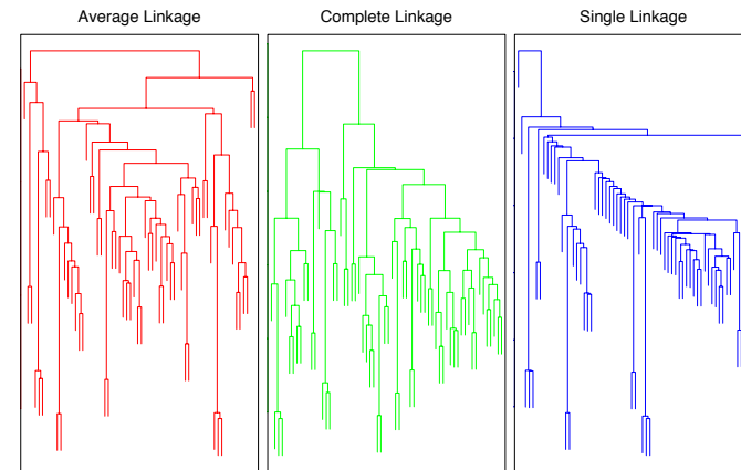
Figure 14.13: Dendrograms from agglomerative hier-
