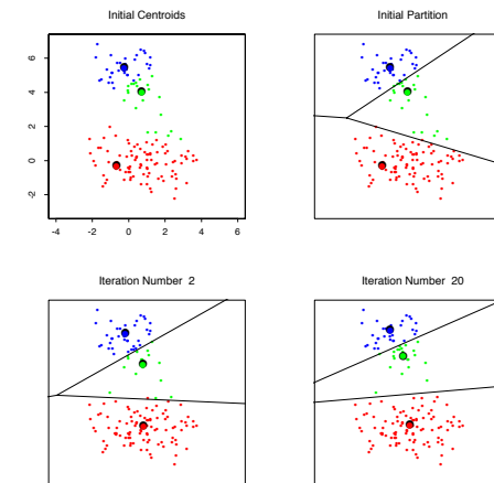
Figure 14.6: Successive iterations of the K-means clustering algorithm for the simulated data of Fig-14.5
